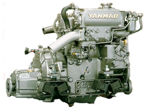
2GM20F Marine Engine
