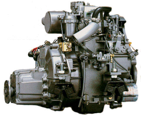
1GM10 Marine Engine
